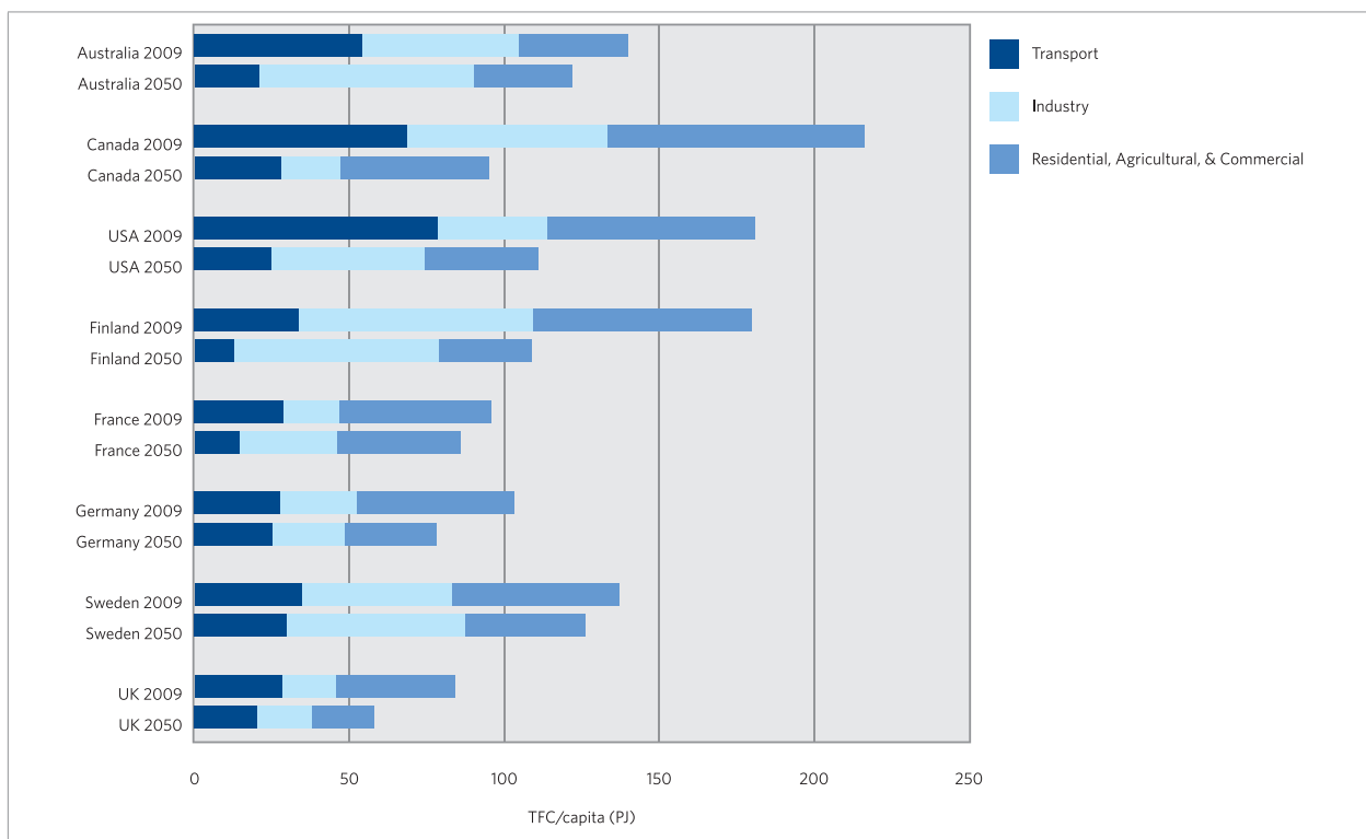
Figure 3. Per Capita Energy Consumption (2009 vs. Scenario)
