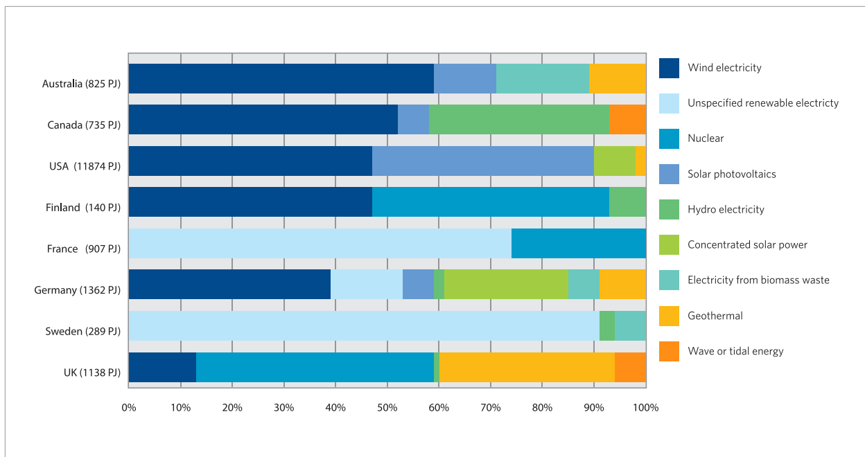
Figure 5. Composition of Carbon-Free Electricity Increase (2009-2050) in Low-Carbon Scenarios
